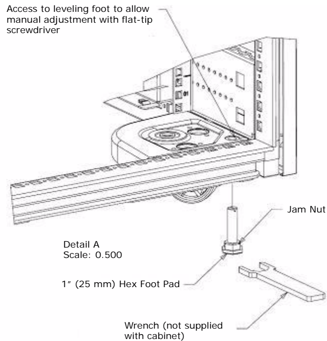
Figure 3-22: Example of Leveling Feet
