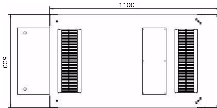
Figure 3-35: Top View (EMEA Rack)
