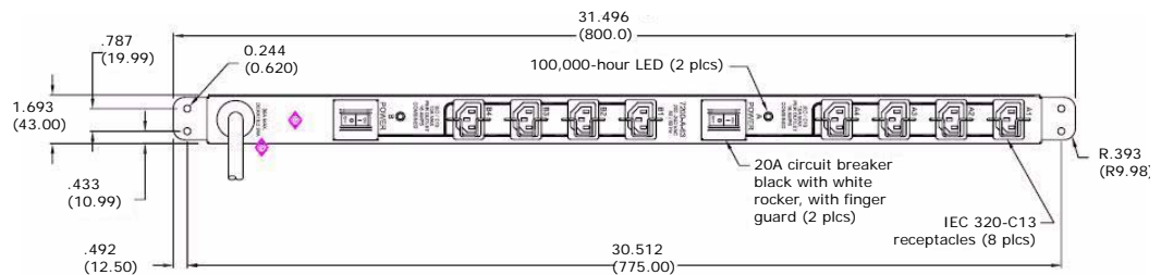
Figure 3-6: Hitachi AMS 2000 Family Rack PDU Design
