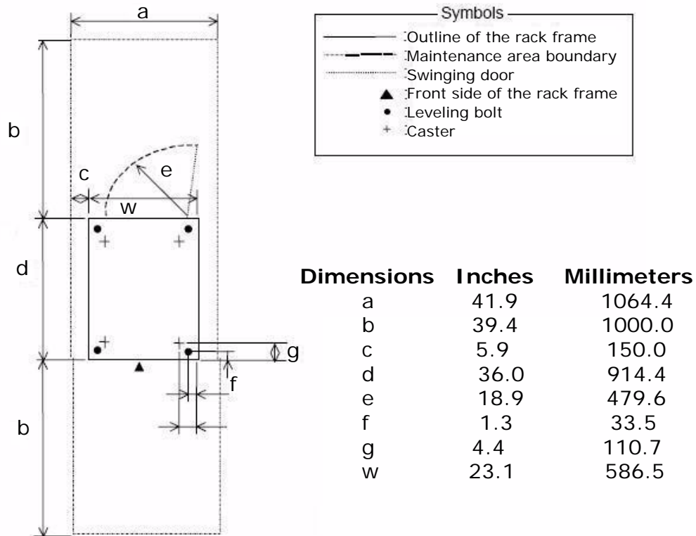
Figure 3-5: Installation and Maintenance Areas
