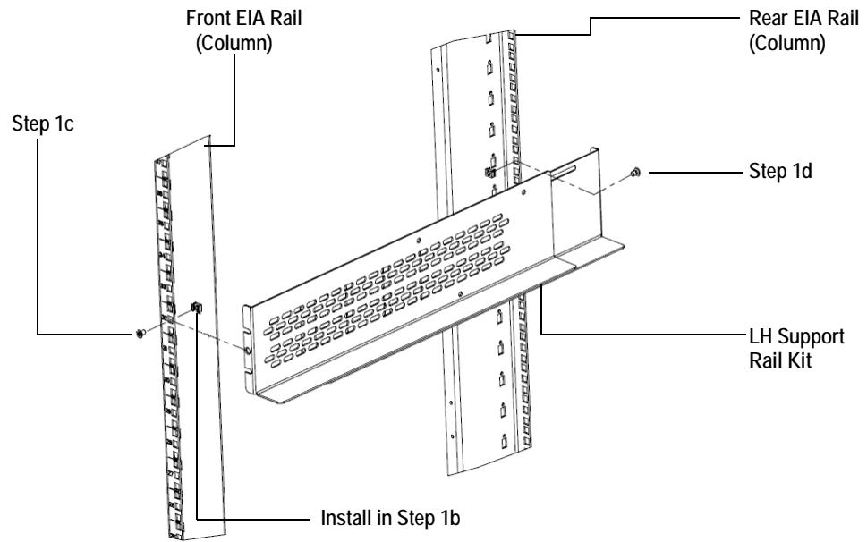
Figure 3-18: Installing the Rack-Mount Rail Kit Rail Assembly, Left Side Shown
