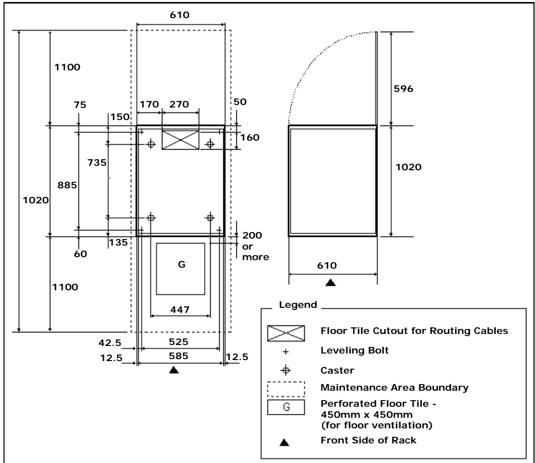
Figure 4-1: Service Clearance Areas
