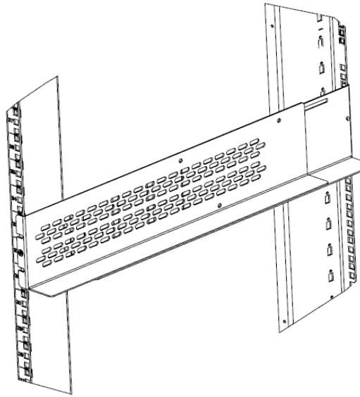
Rail Assembly
