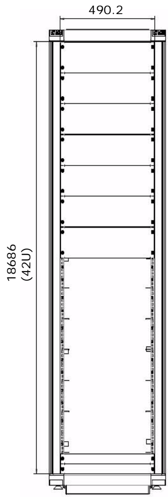
Figure 3-33: Front View (EMEA Rack)
