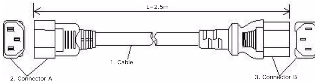
Figure 3-9: Power Jumper Cable (250 VAC 10A IEC320-C14)
