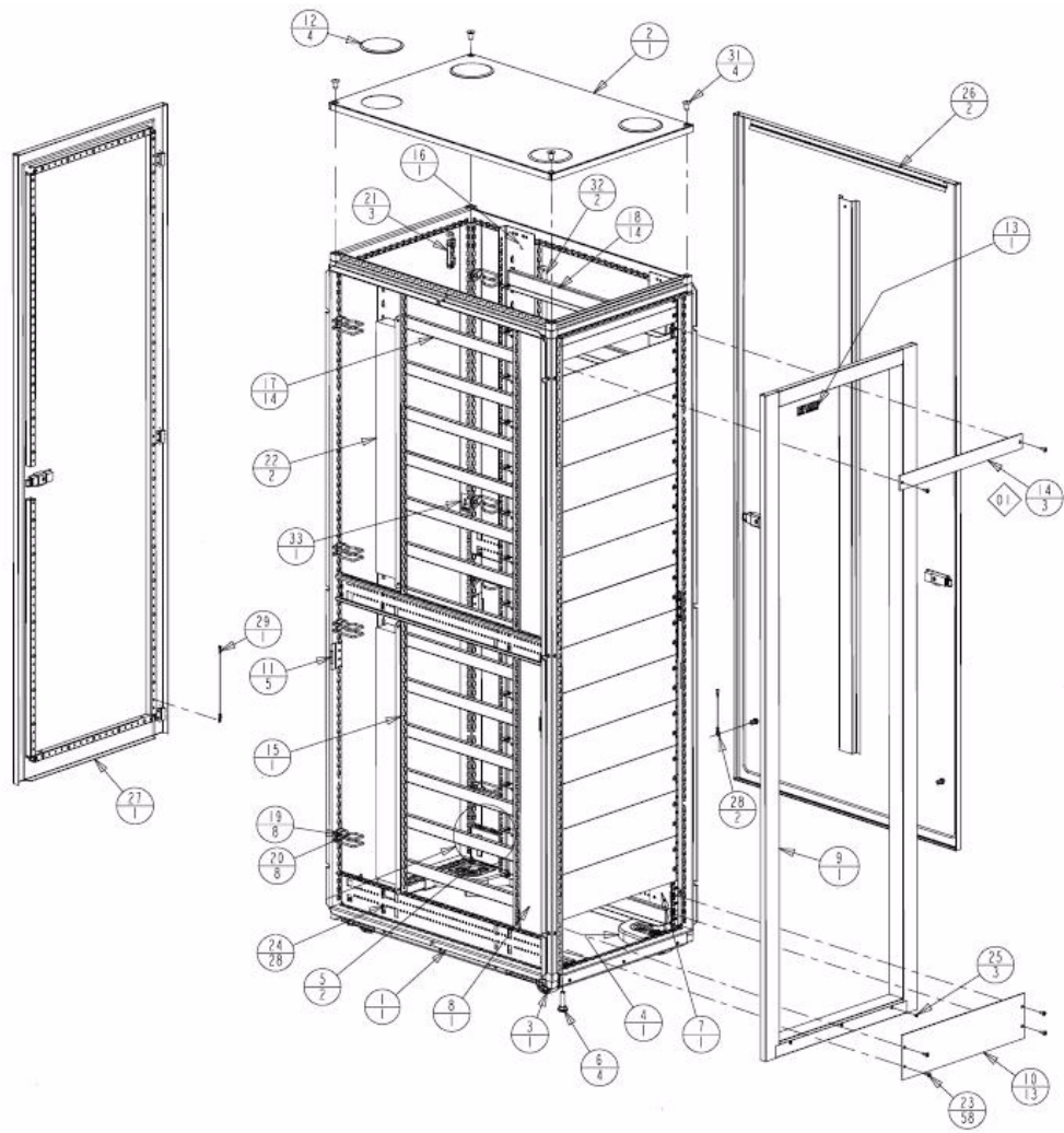
Figure 3-4: Exploded View of the Hitachi AMS 2000 Rack
