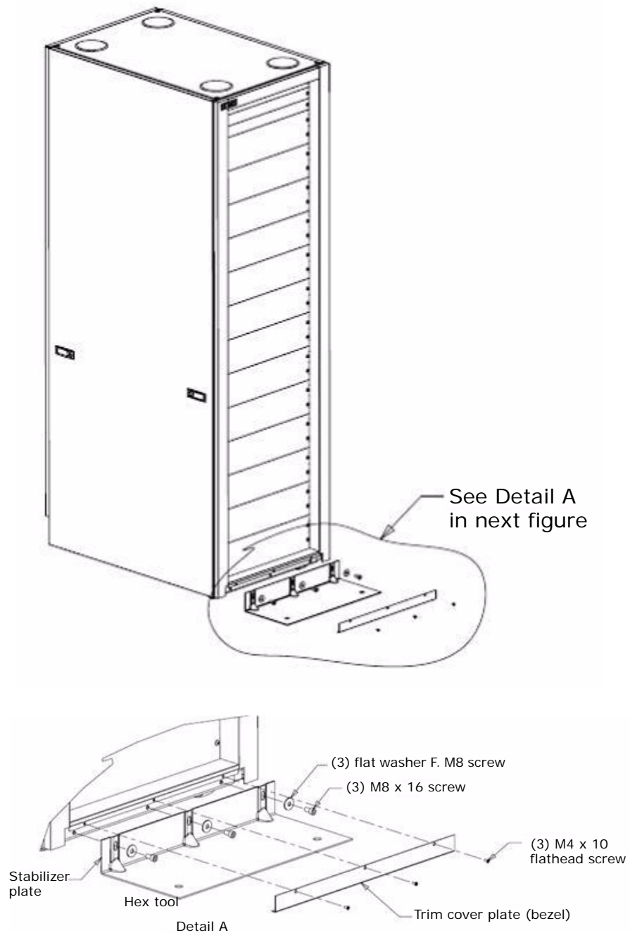
Figure 3-31: Installing and Uninstalling the Anti-Tip Stabilizing Plate
