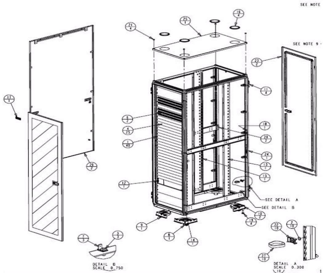
Figure 3-12: Exploded View of the Hitachi Full-Height Solutions Rack
