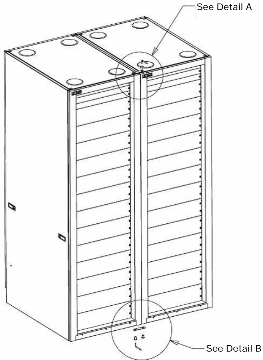
Figure 3-27: Baying Kit
