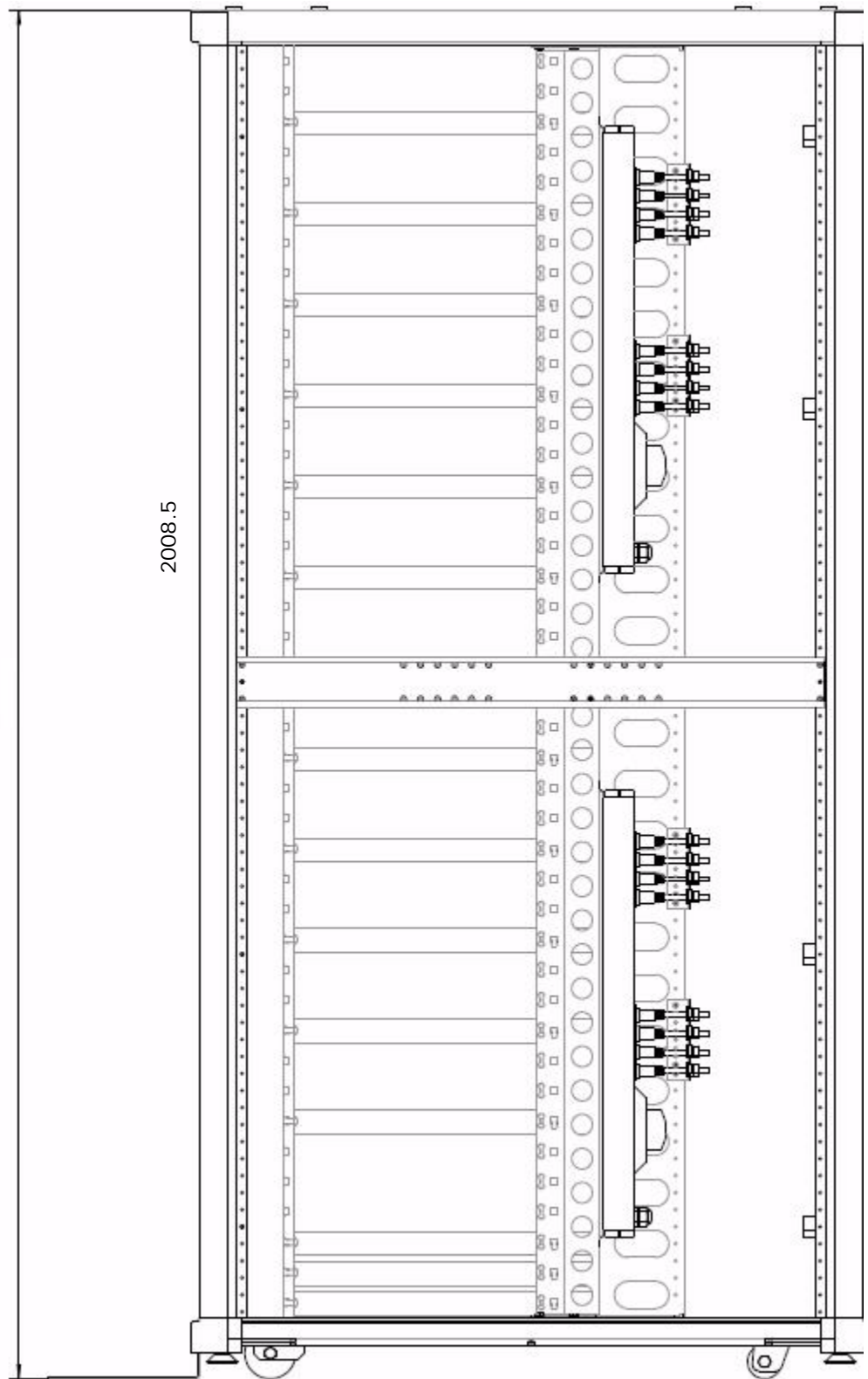
Figure 3-34: Detailed View (EMEA Rack)
