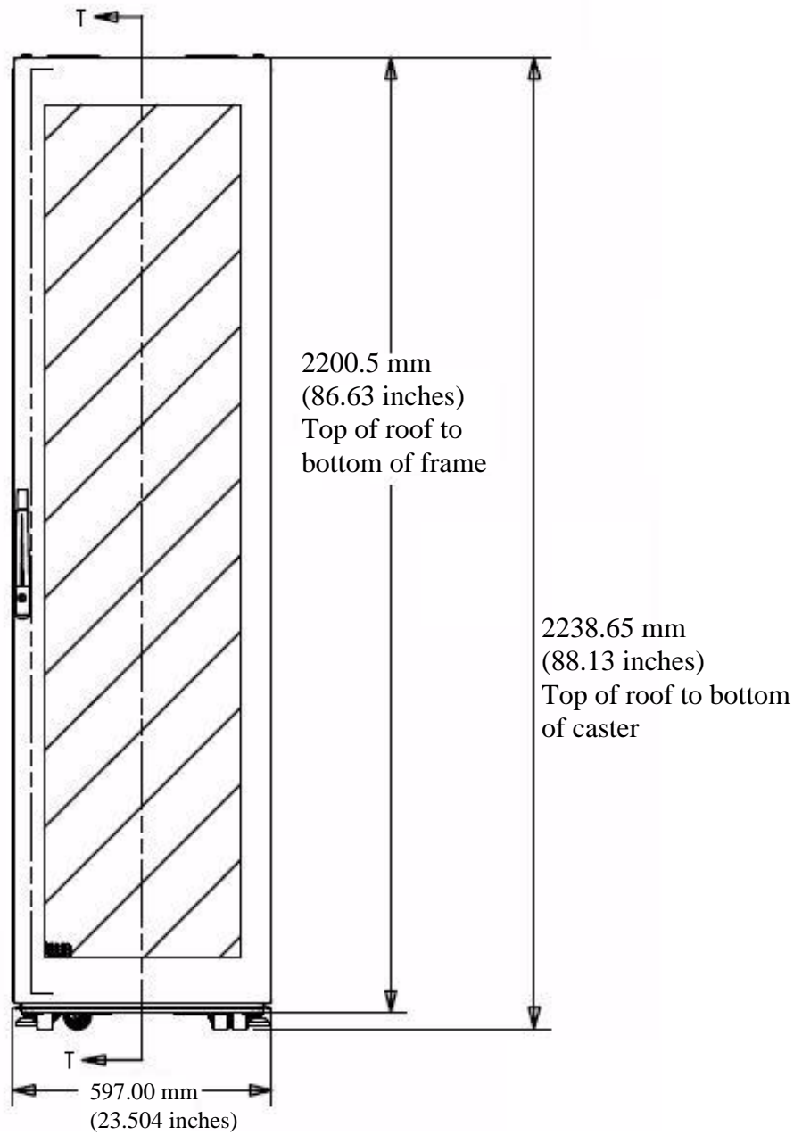
Figure 3-15: Front View of Hitachi AMS 47U Rack
