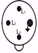
IEC 309 60A Pin and Sleeve Connector
