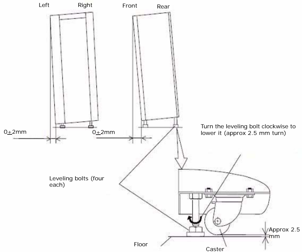
Figure 3-23: Example of Lowering the Leveling Feet
