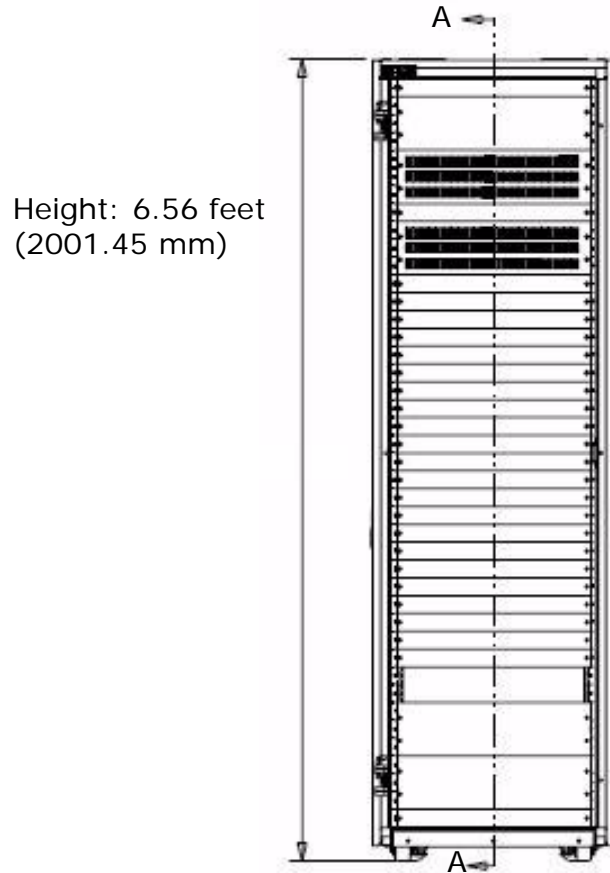
Figure 3-10: Front of the Hitachi Full-Height Solutions Rack (Door Not Shown for Clarity)
