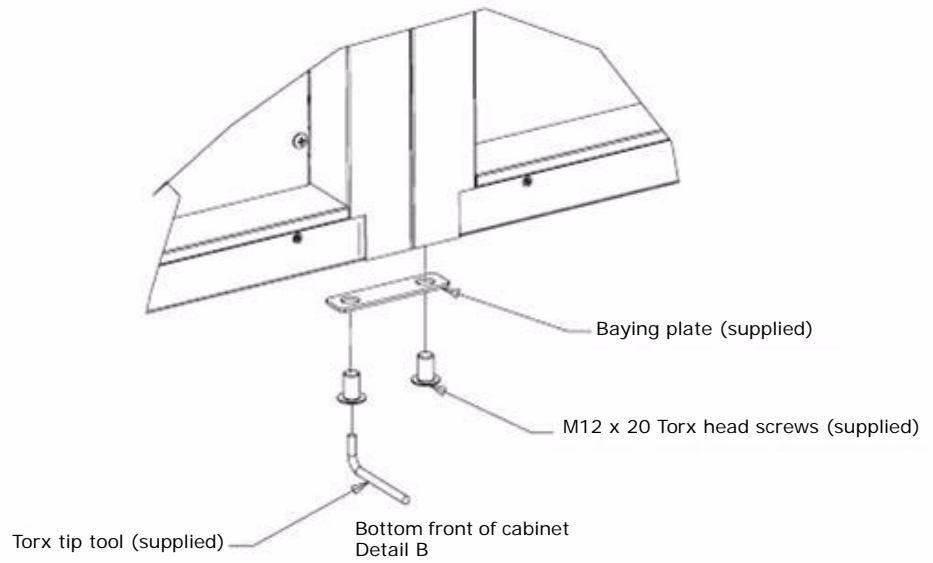
Figure 3-28: Baying Kit (Details A and B) (continued from previous page)
