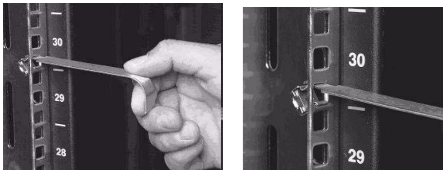
Figure 3-30: Installing the Cage Nuts
