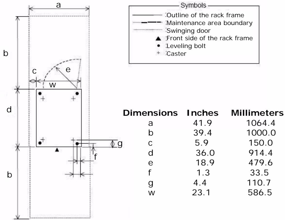
Figure 3-13: Installation and Maintenance Areas
