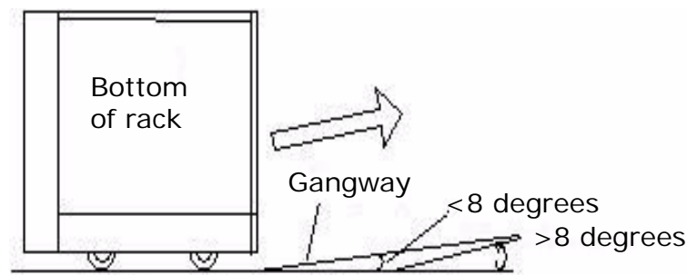
Figure 3-26: Maximum Incline (Slope) for Moving the Rack
